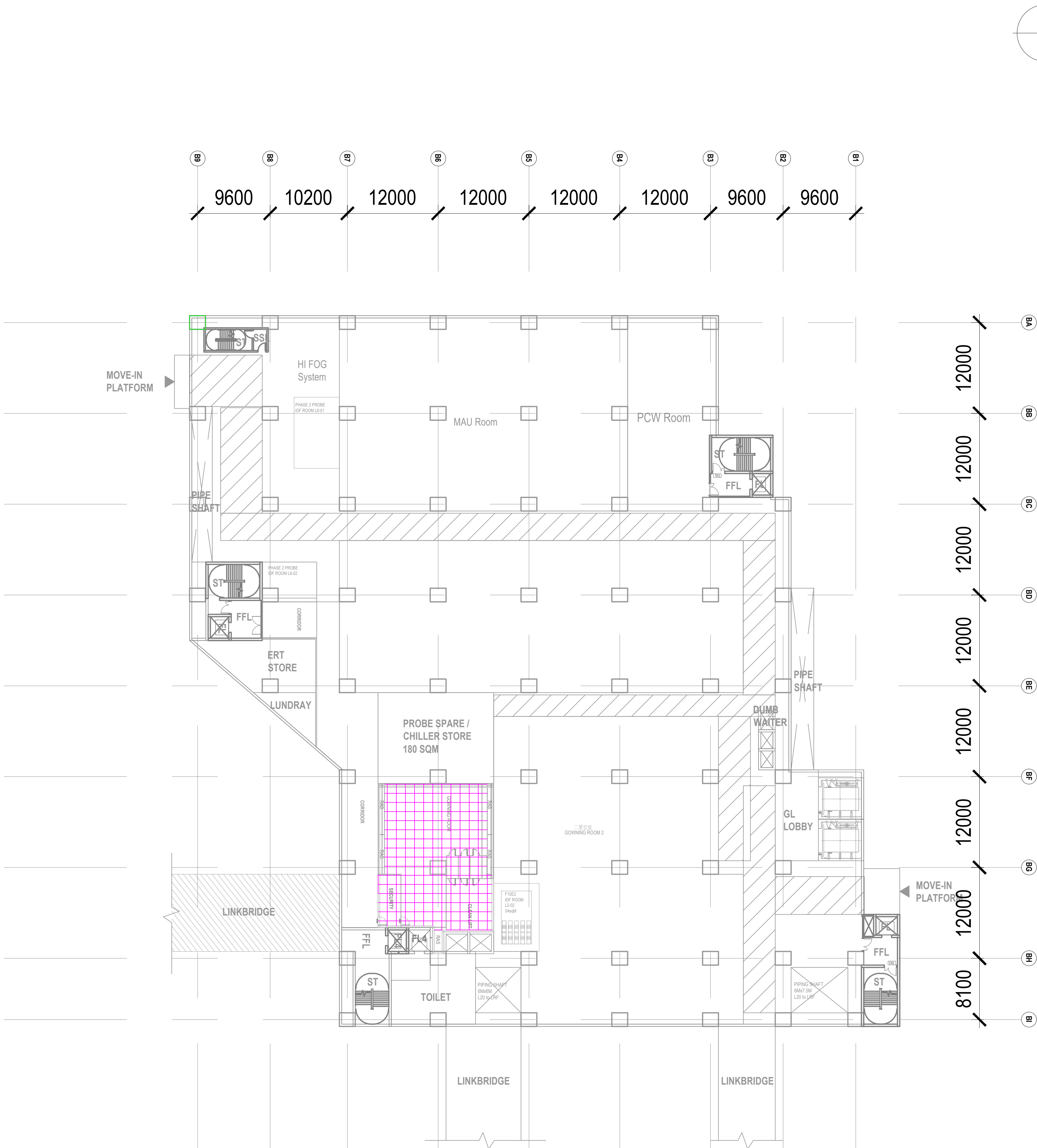
F10E2 L20 CEILING LAYOUT SCALE 1:300
